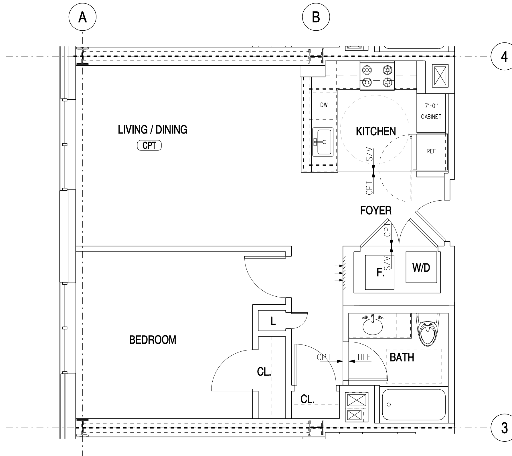
1 TYPICAL ONE BEDROOM SCALE: 1/4"=1'-0"
